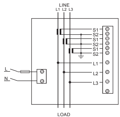
3-Phase 3-Wire up to 600V For two CTs only, see the diagram below
