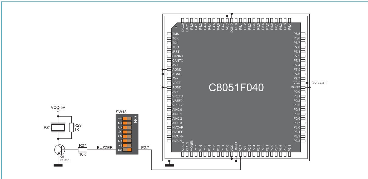
Figure 5-2: Piezo buzzer connected to the microcontroller pin P2.7
