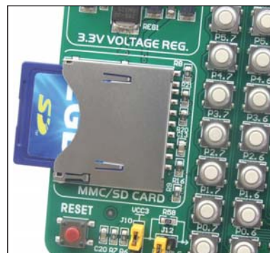
Figure 11-2: MMC/SD connector
