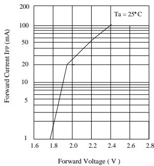
Forward Voltage vs. Forward Current
