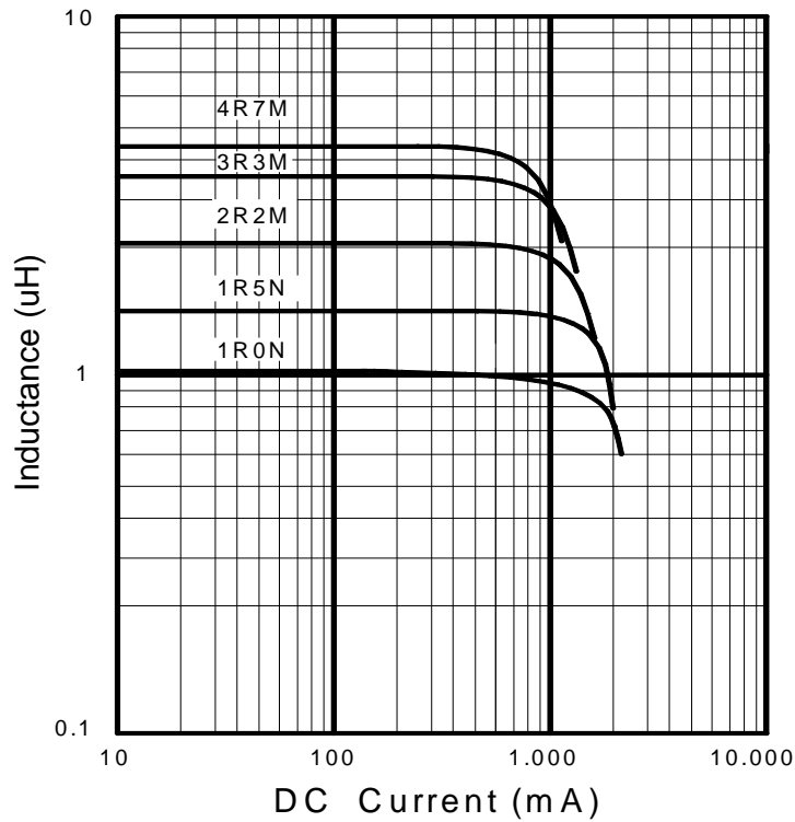
Inductance vs. DC Current
