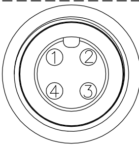
Conn.1 & Conn.2 Pin Assignments Front View
