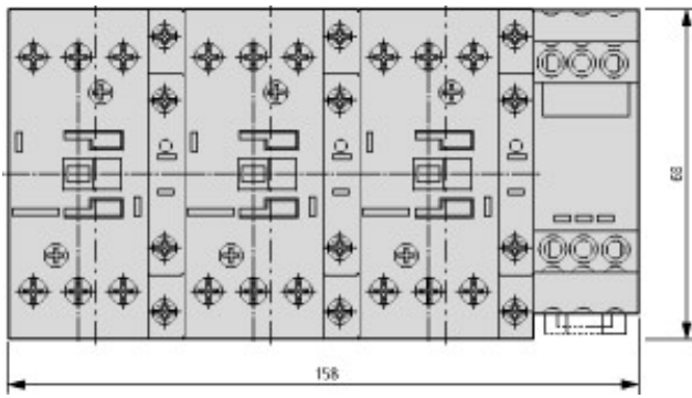
Basic unit with auxiliary contact module
