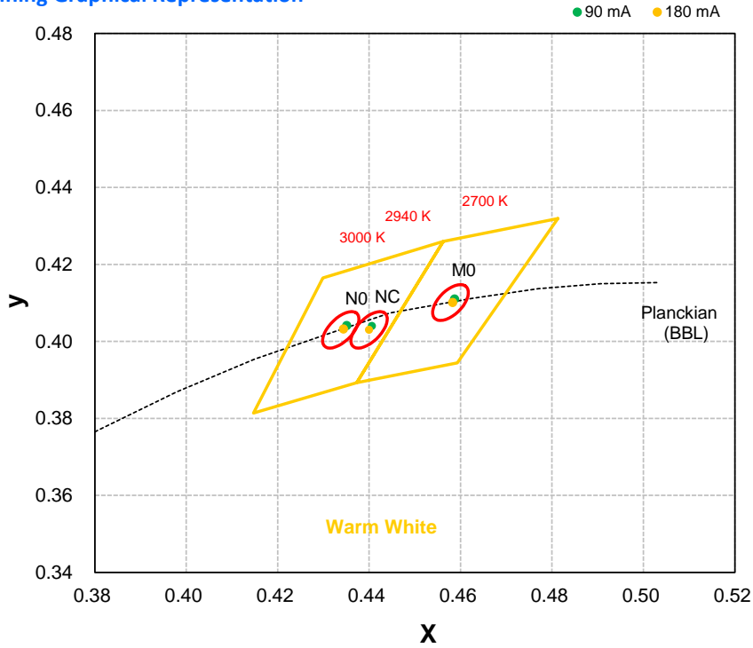
Warm White Binning Graphical Representation
