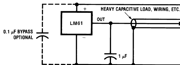
Figure 16. LM61 with Filter for Noisy Environment
