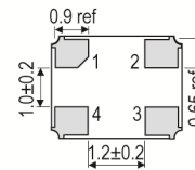
Underside View
