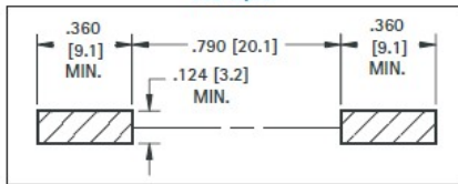
Pad Layout
