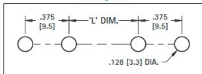
Mounting Detail
