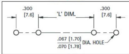
Mounting Detail
