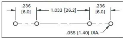
Mounting Detail
