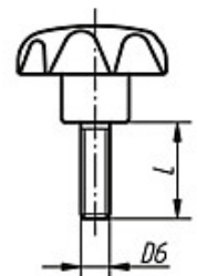
Form L with external thread
