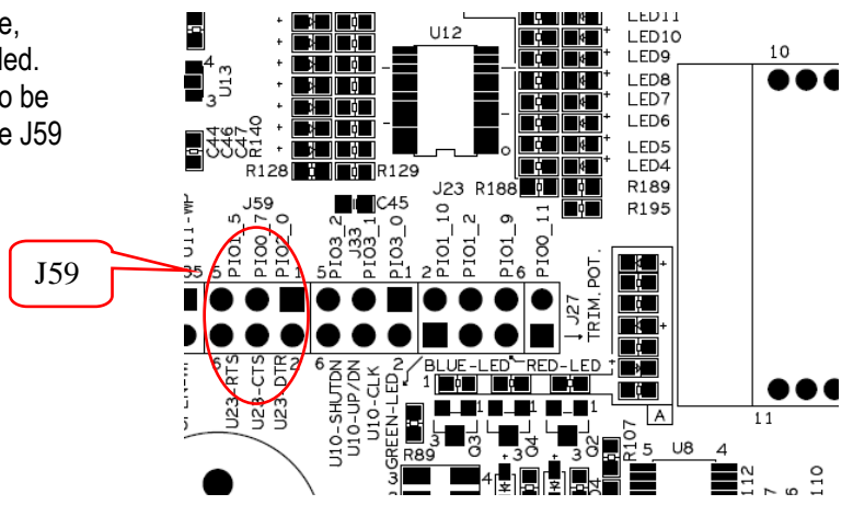
Figure 29 – Jumper Setting: RF-module extra signals
