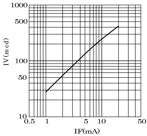
IV-IF Characteristics
