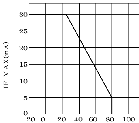
IF Max-Ta Characteristics
