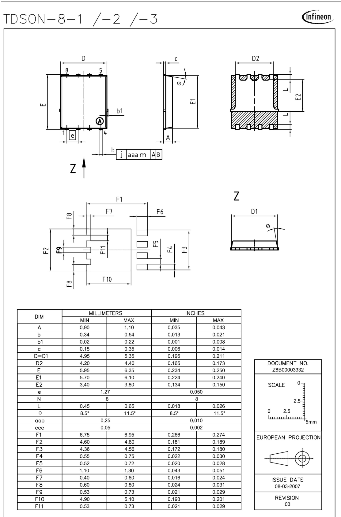
Figure 1 Outline PG-TDSO N -8, dimensions in mm/inches
