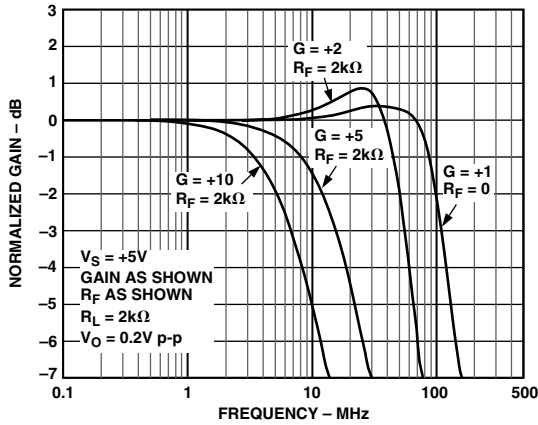
TPC 1. AD8051/AD8052 Normalized Gain vs. Frequency; V_S = +5V
