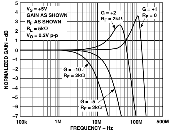
TPC 4. AD8054 Normalized Gain vs. Frequency; V_S = +5V
