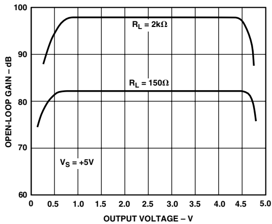
TPC 26. Open-Loop Gain vs. Output Voltage
