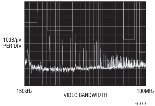
Figure 18. VIN 26.5V, VOUT 3.3V, IOUT 5A, π Filter 20µF to 0.22µH Vishay (1616BZ) to 20µF CISPR25 Conducted Emissions
